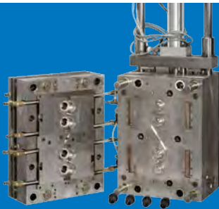
Unscrewing Molds
